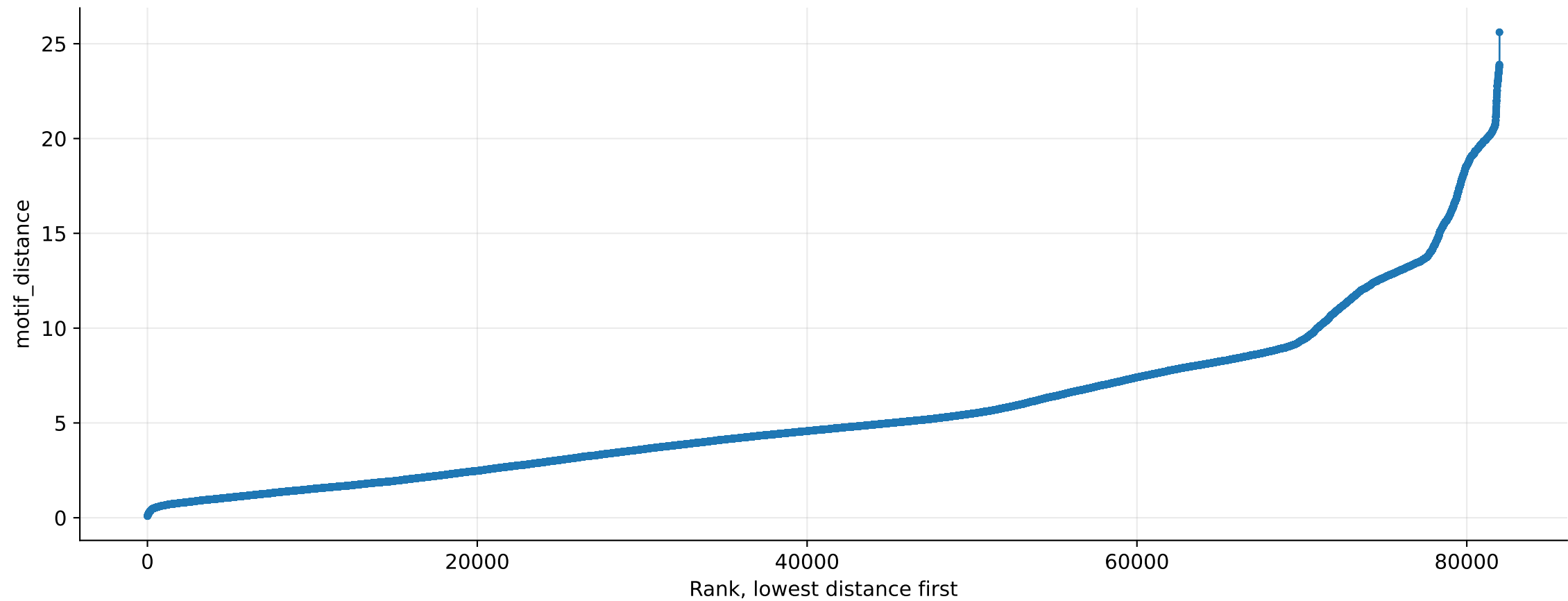
Ranked Matrix Profile motif distances
